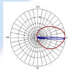
GSM1800 2 DEGREE DOWN TILT
