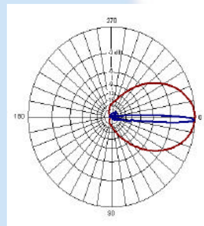
2 DEGREE DOWN TILT PLOT
